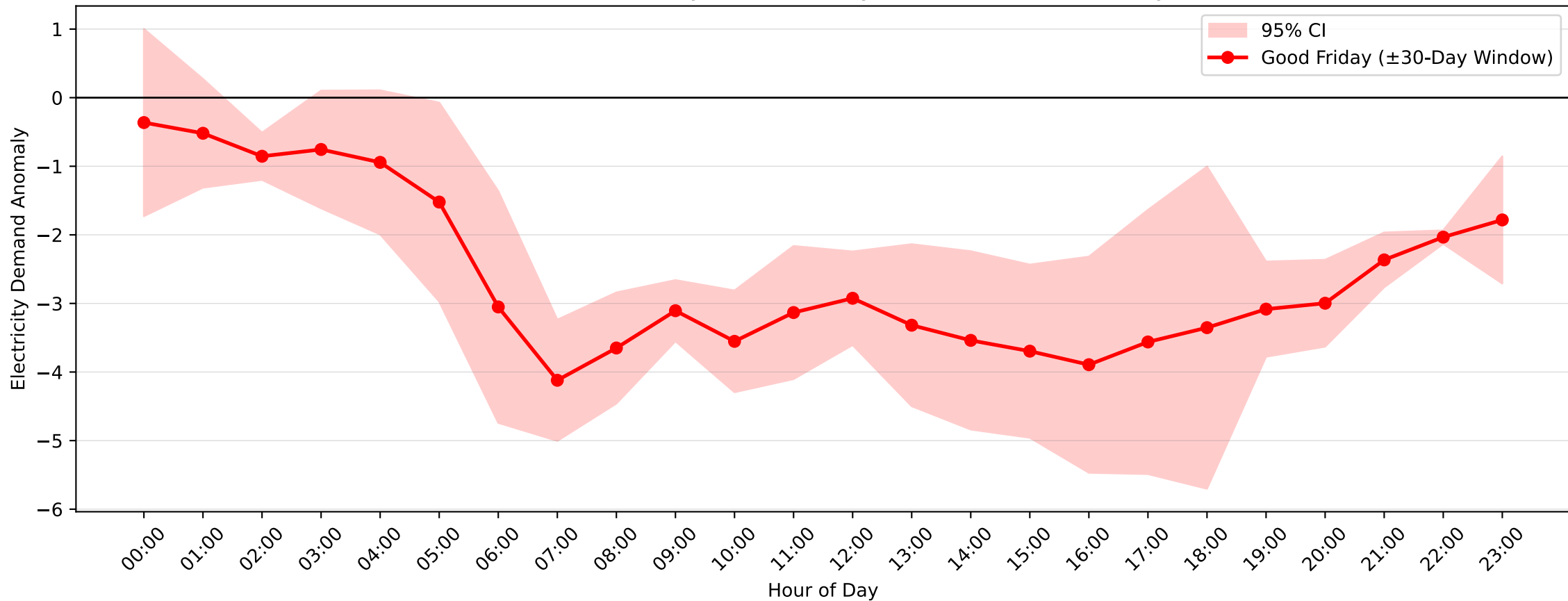
Bass Hill Demand Anomaly: Good Friday (2005–2006, \pm 30 -Day Window)
