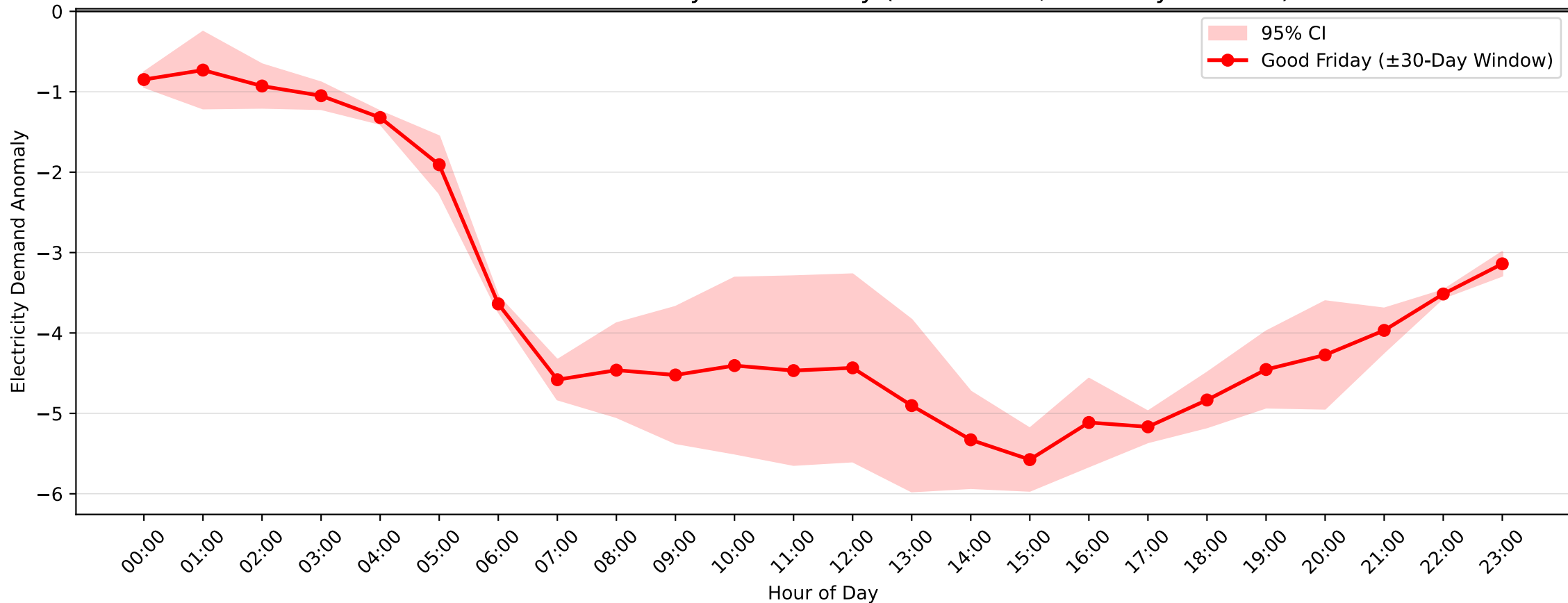
Bass Hill Demand Anomaly: Good Friday (2016-2017, \pm 30 -Day Window)
