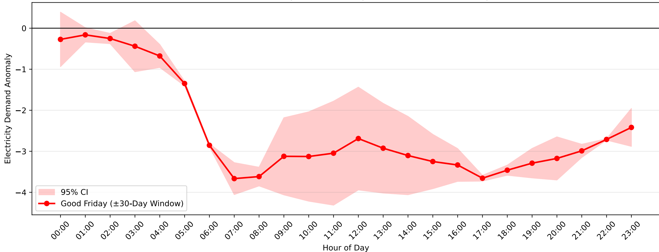
Bass Hill Demand Anomaly: Good Friday (2014–2015, \pm 30 -Day Window)
