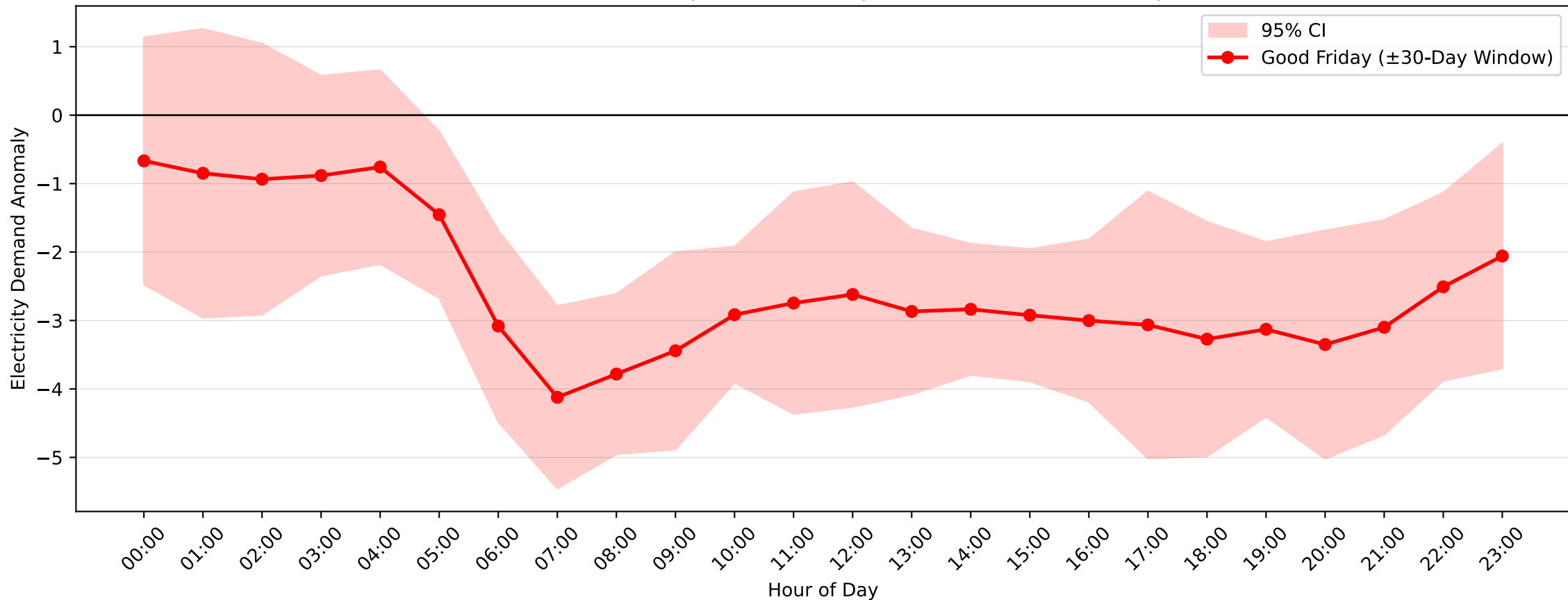
Bass Hill Demand Anomaly: Good Friday (2011-2012, \pm 30 -Day Window)
