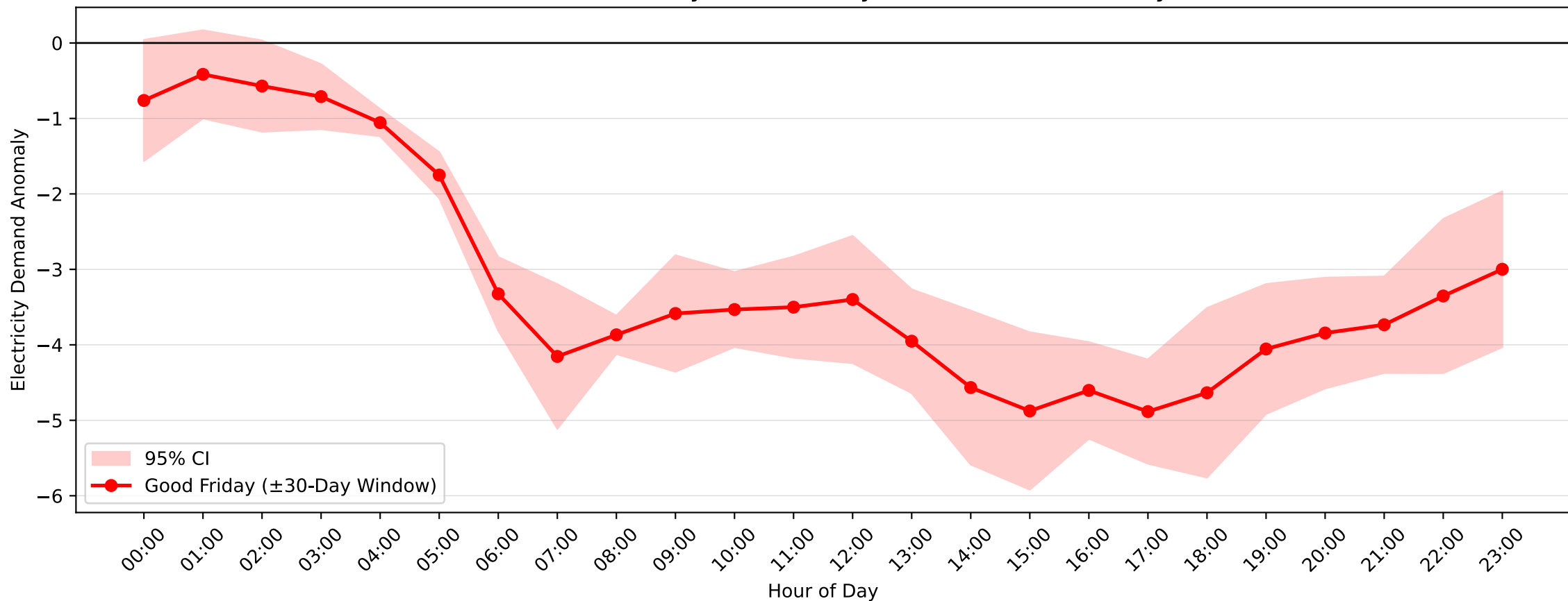
Bass Hill Demand Anomaly: Good Friday (2015–2016, \pm 30 -Day Window)
